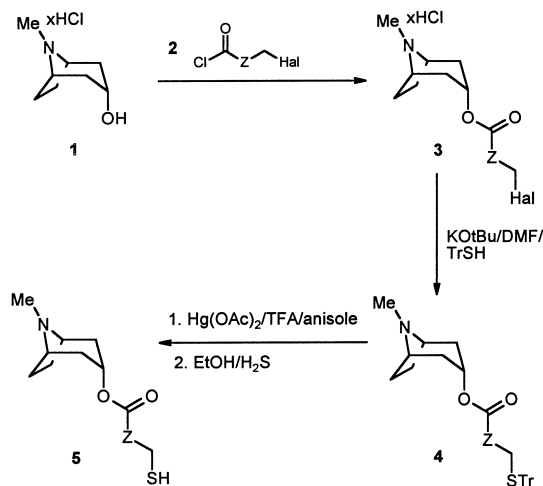
Scheme 1. Synthesis of ω-mercaptoesters of tropane. Z: a = 0, b = CH 2 , c = C 2 H 4 , d = C 3 H 6 , e = C 4 H 8 , f = 1,3-phenyl, g = 1,4-phenyl.
